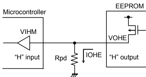
Fig 43. DO pull down resistance
