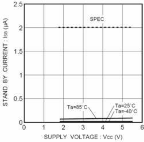
Figure 18. Consumption current at standby action IBS
