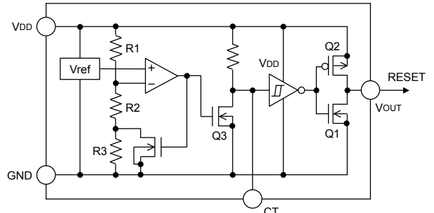
Figure.16 (BD53ExxxType Internal Block Diagram)
