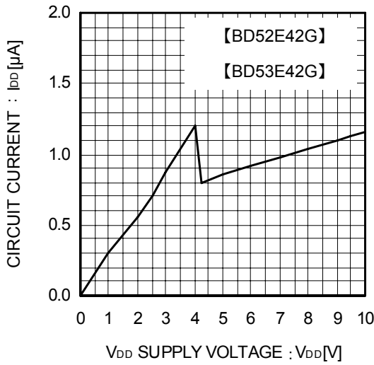
Figure.3 Circuit Current
