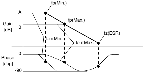
Fig.99 Open loop gain characteristics
