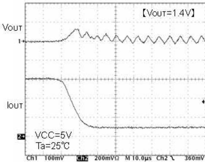
Fig.69 Transient response I_o=600\rightarrow 100mA(10\mu s)
