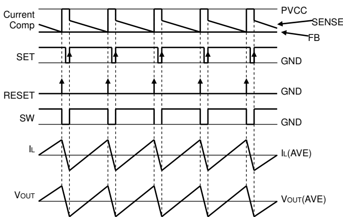
Fig.85 Diagram of current mode PWM control
