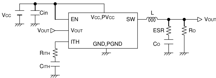
Fig.101 Typical application
