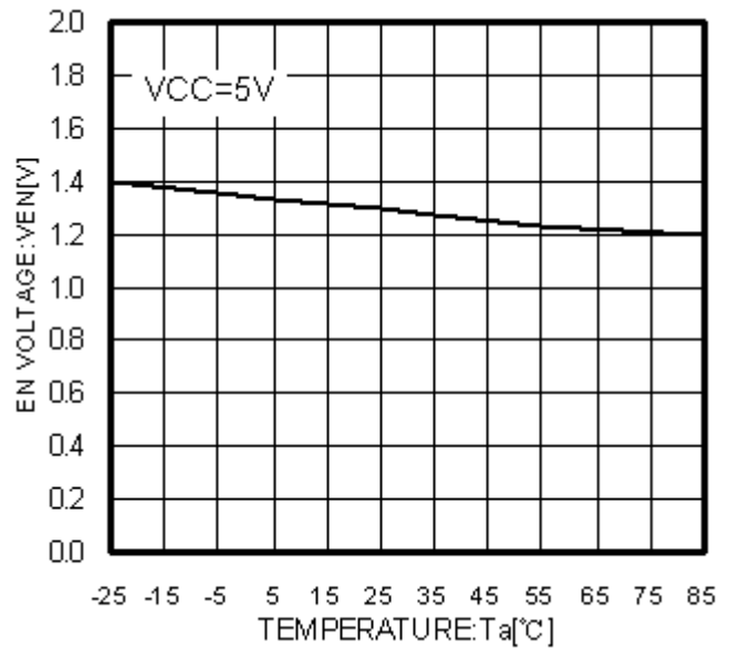
Fig.32 T_a - V_{EN}
