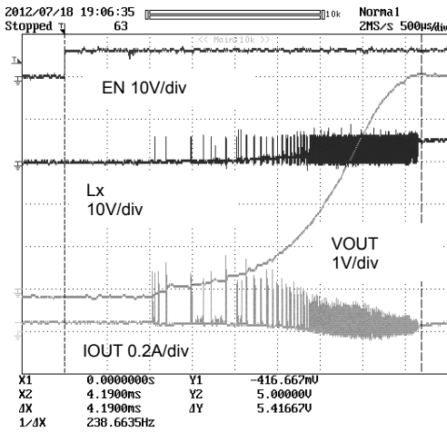
Figure 19. Start-up Characteristics VIN=8V, IOU=0mA, VOUT=5V
