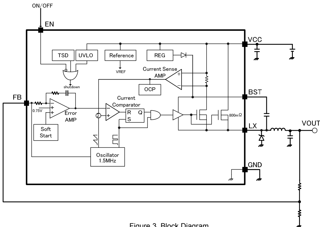
Figure 3. Block Diagram
