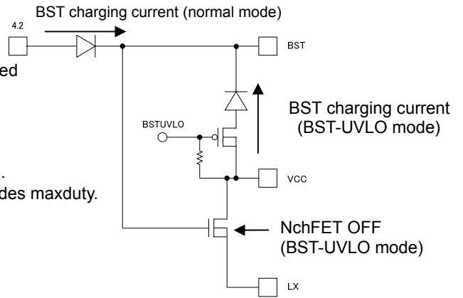
Figure 4. BST-UVLO image
