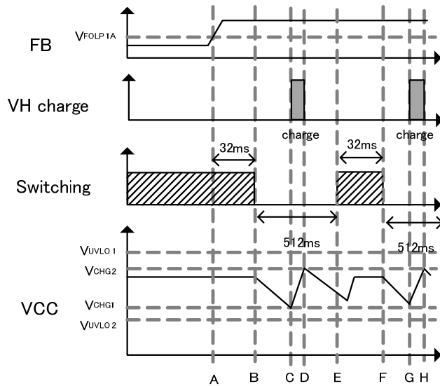
Figure 15. Over load protection (Auto recovery)
