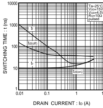
Fig.9 Switching Characteristics
