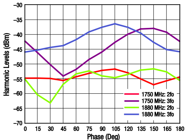
Figure 15. Harmonics vs Phase (ANT to GSM_TX_HB, P_{\text{IN}} = +33 \text{ dBm} , 5:1 VSWR Mismatch)
