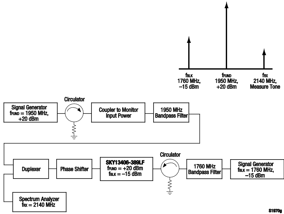
Figure 16. 3 rd Order Intermodulation Test Setup
