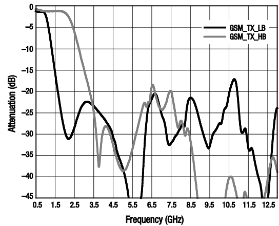
Figure 6. Attenuation vs Frequency (ANT to GSM_TX_HB/LB Ports)
