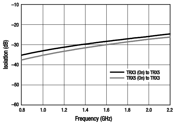
Figure 11. Isolation vs Frequency (TRX3 to TRX5 Ports)
