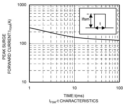
I_{FSM}-t CHARACTERISTICS
