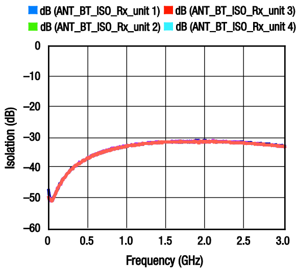
Figure 13. RF2 to RF3 Isolation
