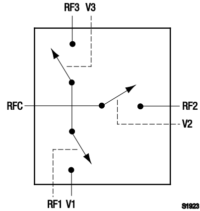
Figure 1. SKY13309-370LF Block Diagram
