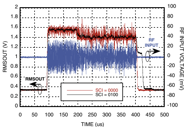
Residual Ripple for 2.6 GHz WiMAX OFDM Advanced 802.16 @ SCI = 0100
