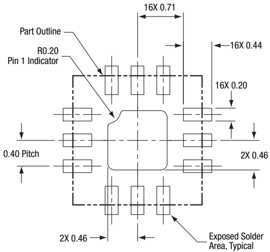
Figure 14. SKY13346-368LF PCB Layout Footprint (Top View)
