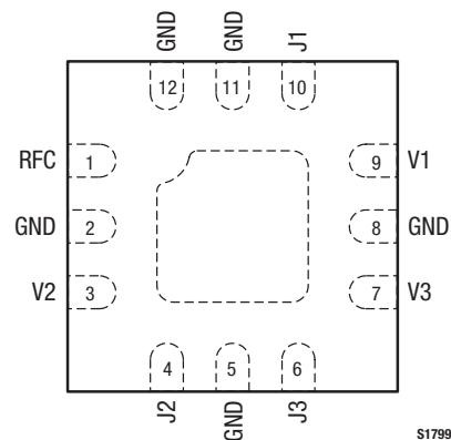
Figure 2. SKY13346-368LF Pinout – 12-Pin QFN (Top View)
