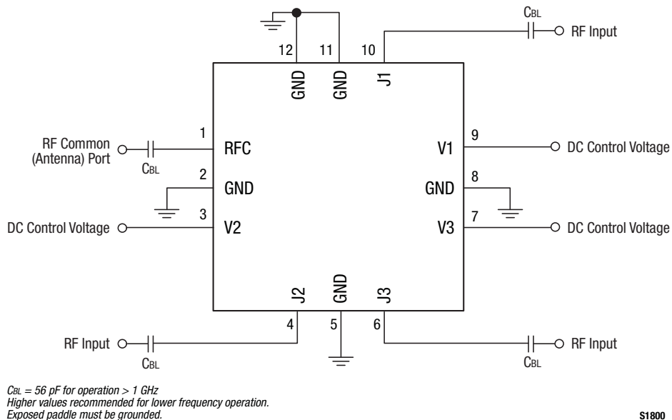
Figure 12. SKY13346-368LF Evaluation Board Schematic
