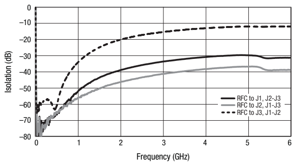
Figure 7. Port to Port Isolation vs Frequency (Off Ports to Off Ports)
