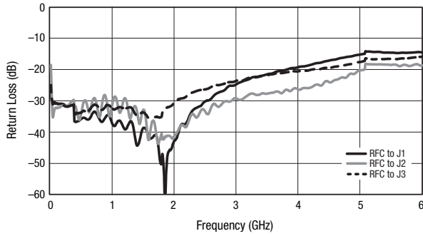
Figure 9. Input Return Loss vs Frequency
