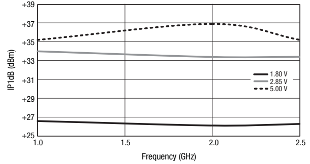
Figure 10. Input 1 dB Compression Point vs Frequency
