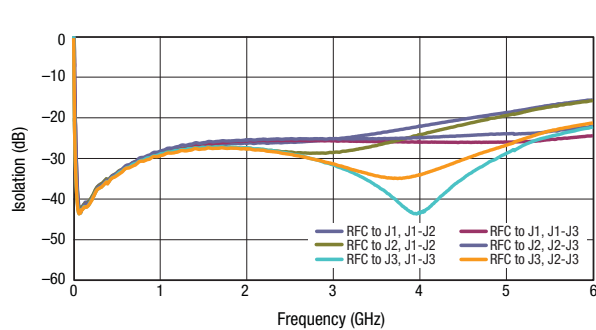
Figure 8. Port to Port Isolation vs Frequency (Insertion Loss Ports to Off Ports)
