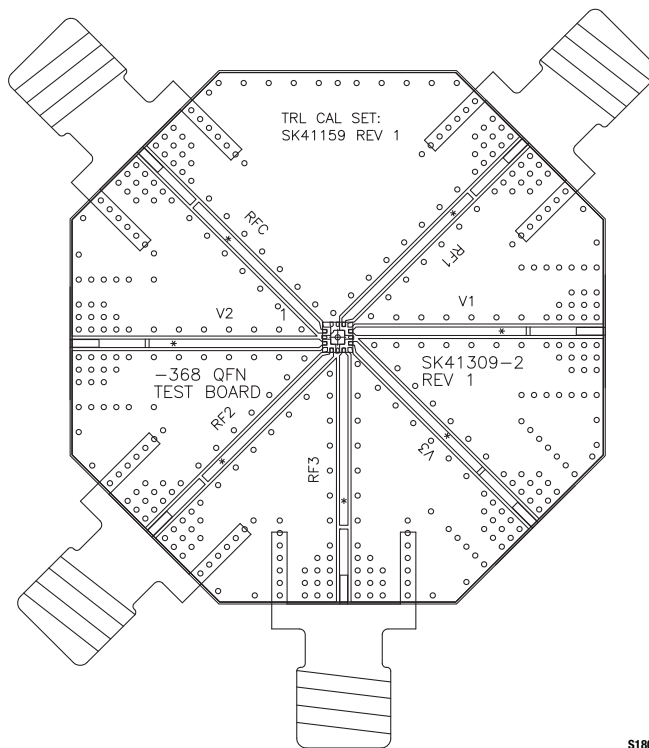
Figure 13. SKY13346-368LF Evaluation Board Assembly Diagram
