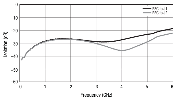
Figure 6. Isolation vs Frequency (RFC to J3 Insertion Loss State)
