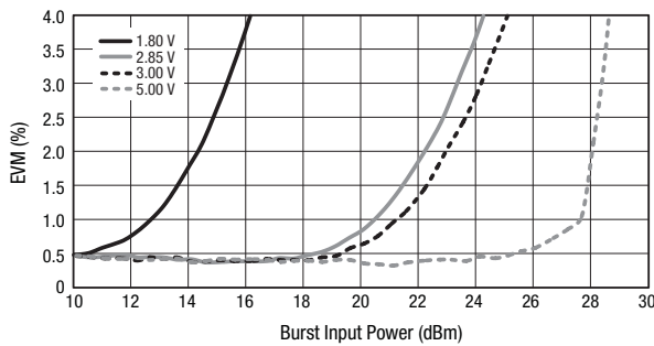
Figure 11. EVM vs Burst Input Power Over Voltage (F = 2.5 GHz, 802.11g, 54 Mbps, 64 QAM)
