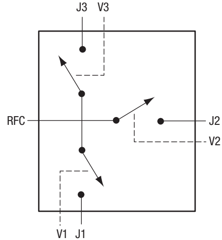
Figure 1. SKY13346-368LF Block Diagram
