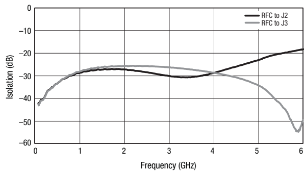
Figure 4. Isolation vs Frequency (RFC to J1 Insertion Loss State)
