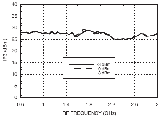
Input IP3 vs. LO Drive, IF = 240 MHz [1]
