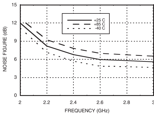
Noise Figure vs. Temperature, Vs= 3.6V
