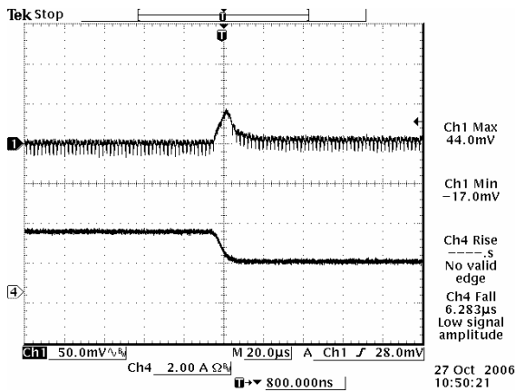
100% to 50% load step at 12 V input, 0.591 V output
