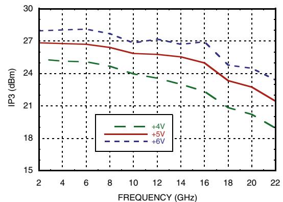
Output IP3 vs. Vdd @ Pout = 4 dBm Tone
