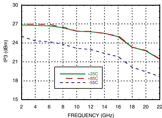
Output IP3 vs. Temperature @ Pout = 4 dBm Tone
