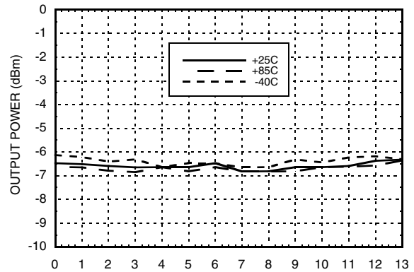
Divide-by-4 Output Power vs. Tuning Voltage, Vcc = +5V
