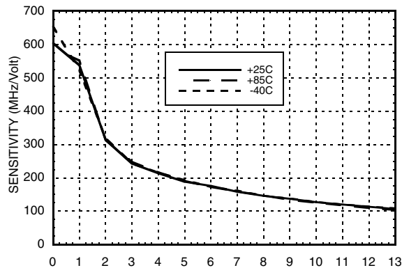
Sensitivity vs. Tuning Voltage, Vcc = +5V
