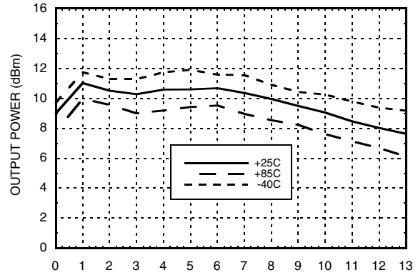
RFOUT/2 Output Power vs. Tuning Voltage, Vcc = +5V
