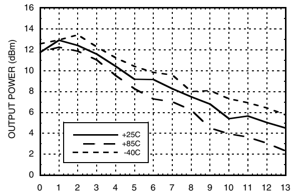
Output Power vs. Tuning Voltage, Vcc = +5V
