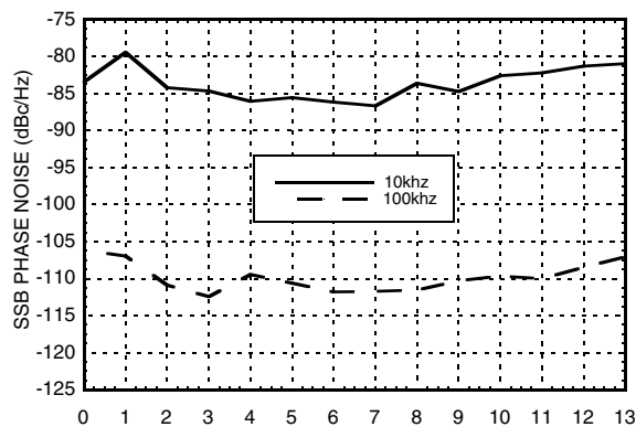
SSB Phase Noise vs. Tuning Voltage
