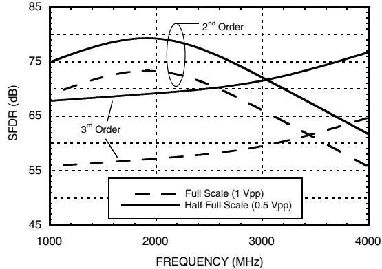
Hold-Mode SFDR vs. Frequency & Input Power [2]
