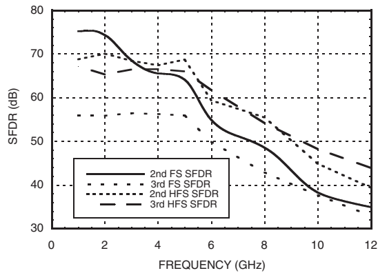
Hold-Mode SFDR vs. Frequency & Input Power @ f_{clk} = 500 \text{ MHz} @ +10 \text{ dBm} [1] [2]
