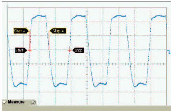
Output Signal [2]
