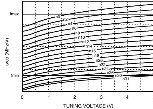
Typical VCO Tuning Curves vs. Switch Position
