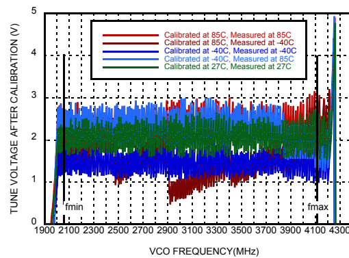
Figure 10. Typical Tuning Voltage After Calibration [6]
