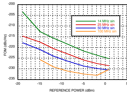
Figure 24. Reference Input Sensitivity, Sinusoidal Wave [17]
