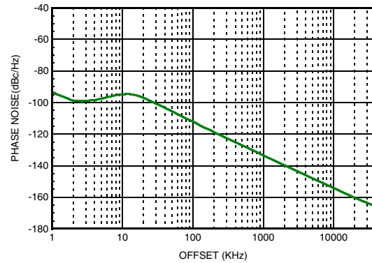
Figure 36. HMC835LP6GE with External VCO HMC384LP4E at 2213MHz [25]
