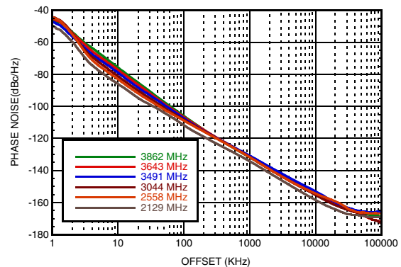
Figure 6. Free Running VCO Phase Noise
