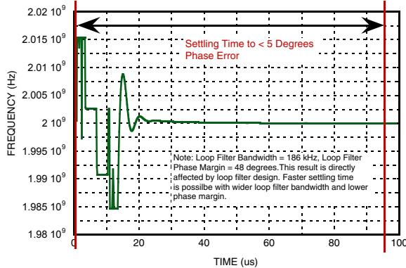
Figure 31. Frequency Settling After Frequency Change, AutoCal Enabled [22]
