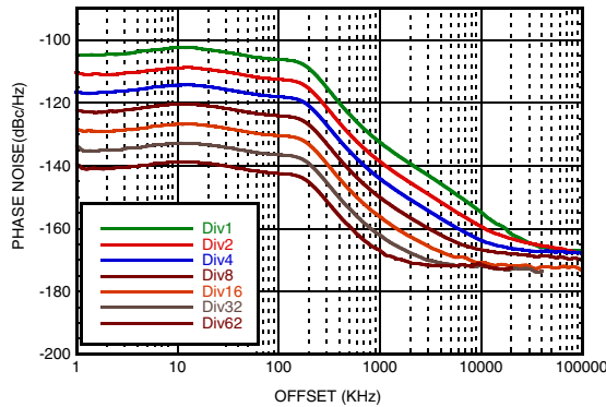
Figure 3. Closed Loop Phase Noise at 3300 MHz, Divided by 1 to 62 [1][5]
