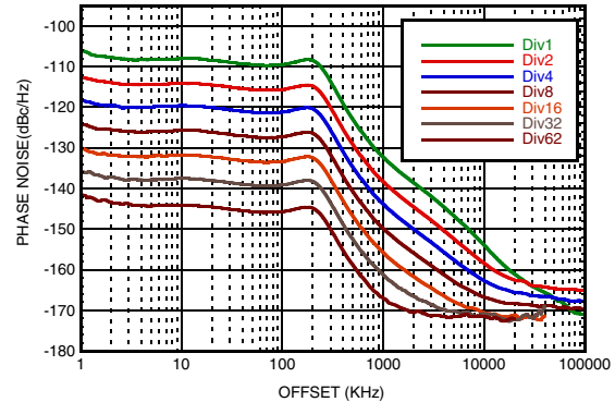
Figure 4. Closed Loop Phase Noise at 3300 MHz, Divided by 1 to 62 [1][5]
