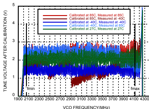
Figure 40. Typical VCO Tuning Voltage After Calibration
