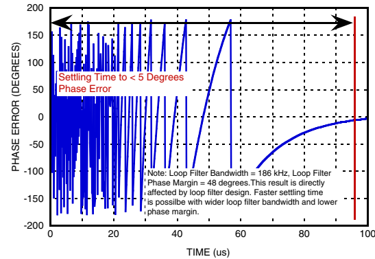
Figure 32. Phase Settling After Frequency Change, AutoCal Enabled [22]
