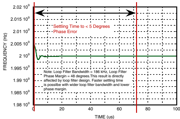
Figure 33. Frequency Settling After Frequency Change, Manual Calibration [23]
