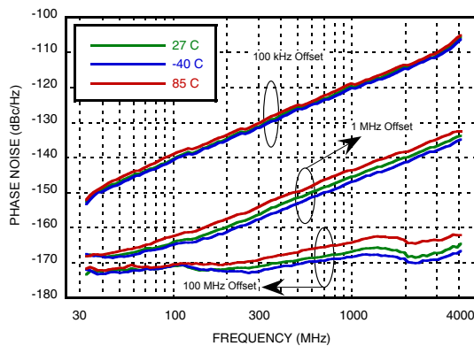
Figure 11. Open Loop Phase Noise vs. Temp
