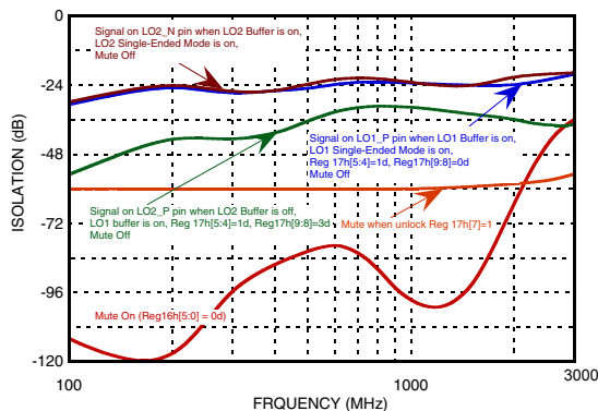
Figure 37. HMC835LP6GE Mute and Isolations
