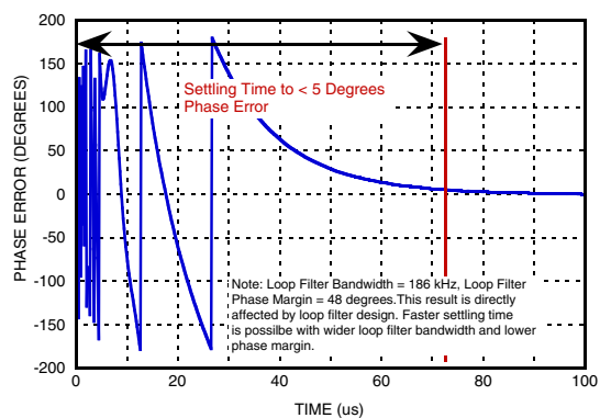
Figure 34. Phase Settling After Frequency Change, Manual Calibration [23]
