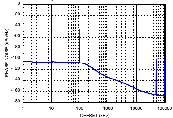
Figure 22. Typical Spurious vs Offset from 3 GHz, Fixed vs. Tunable Reference [16]
