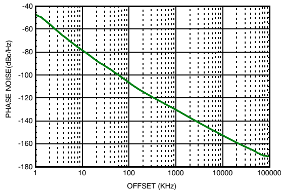
Figure 7. Free Running VCO Phase Noise at 3600 MHz
