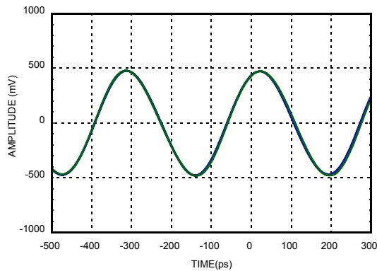
Figure 27. Phase Adjust at 180 degree [20]
