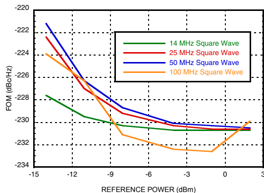
Figure 23. Reference Input Sensitivity, Square Wave [17]
