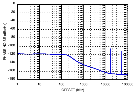
Figure 17. Fractional Spurious Performance at 2646.96 MHz, Exact Frequency Mode ON [11]
