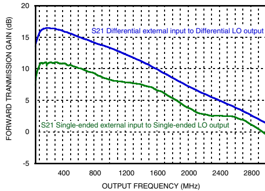
Figure 35. Forward Transmission Gain [24]
