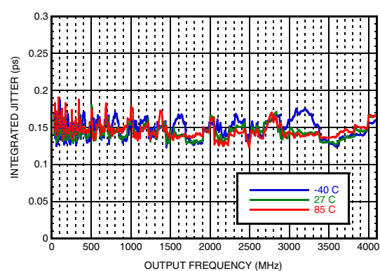
Figure 12. Single Sideband Integrated Phase Noise [7]
