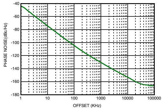
Figure 8. Free Running VCO Phase Noise at 4100 MHz
