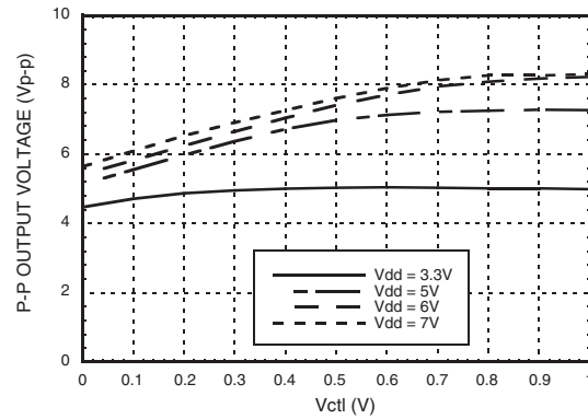
Peak-to-Peak Output Voltage vs. Vctl @ 11.25 Gbps [1]
