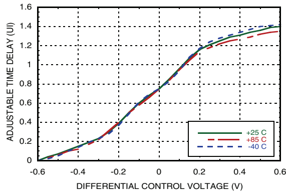
Time Delay vs. Temperature [1][2][3][4]
