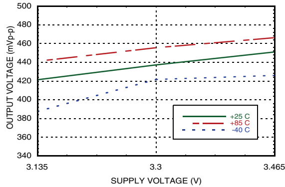
Single-Ended Output Swing vs. Supply Voltage [1][2][3]
