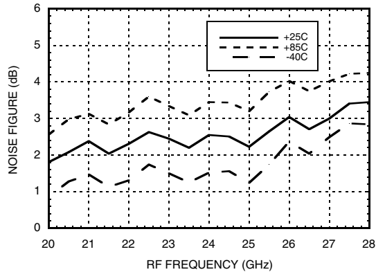
Noise Figure vs. Temperature, IF Frequency = 1000 MHz
