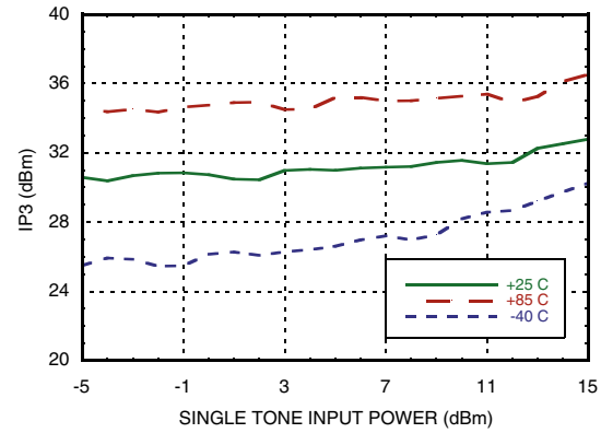
Input IP3 vs. Input Power Over Temperature @ 20 GHz Vct11 = Vct12
