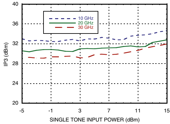
Input IP3 vs. Input Power Over Frequency Vct11 = Vct12
