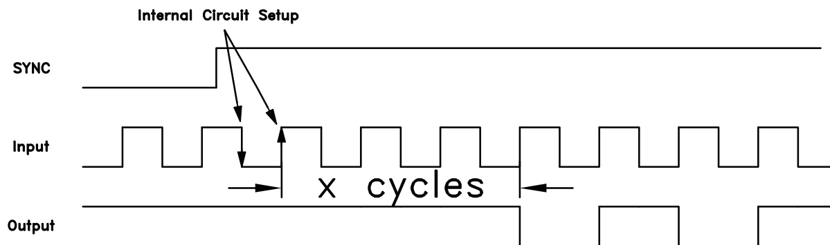
Figure 2. HMC988LP3E SYNC Function Timing Diagram
