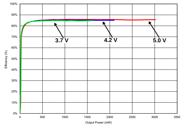
Figure 53. Efficiency vs. Output Power - FHD Mode R_L = 4 \Omega + 33 \mu H
