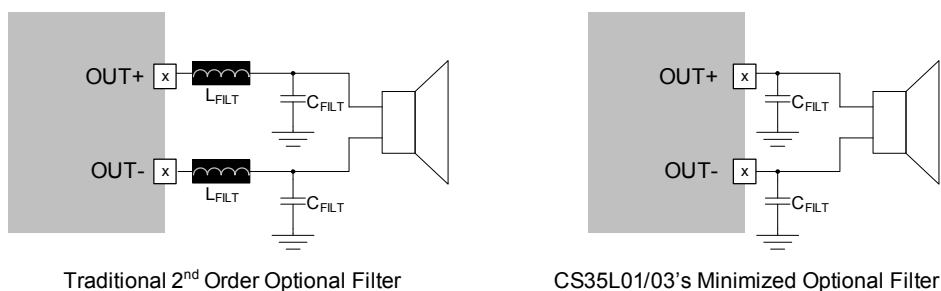
Figure 5. Optional Output Filter Components
