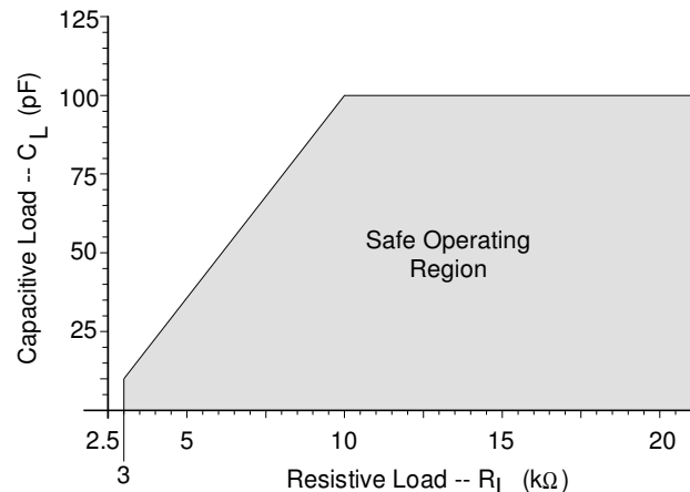
Figure 2. Maximum Loading
