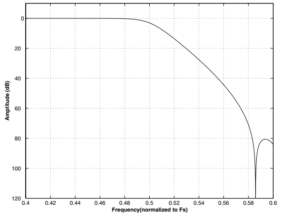
Figure 12. Double-Speed Transition Band
