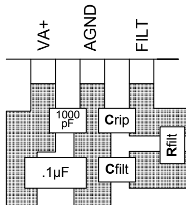
Figure 31. Recommended Layout Example
