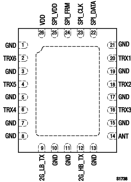
Figure 2. SKY18106-455LF Pinout – 26-Pin QFN (Top View)
