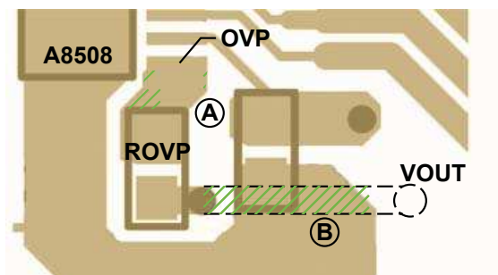
Figure 24. OVP resistor connections; (A) connection should be short, (B) connection to V_{OUT} can be long, and ROVP should be as close to the OVP pin as possible.
