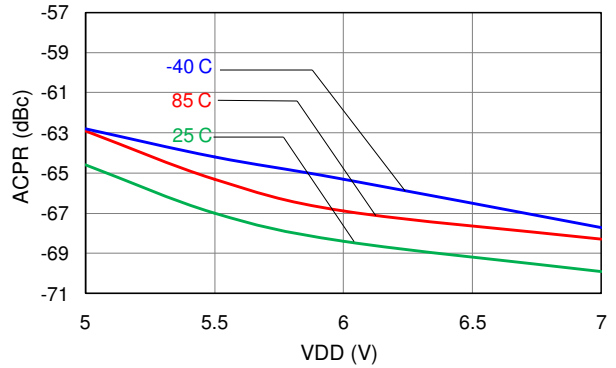
ACPR & Gain
