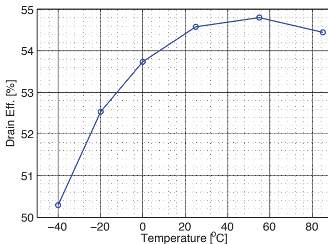
T1G4005528-FS DEff vs. Temp.
