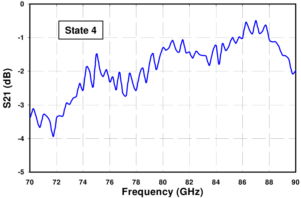
Insertion Loss RF IN to RF OUT 4
