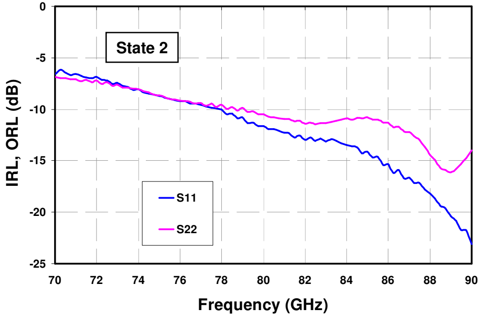
Return Loss RF IN to RF OUT 2
