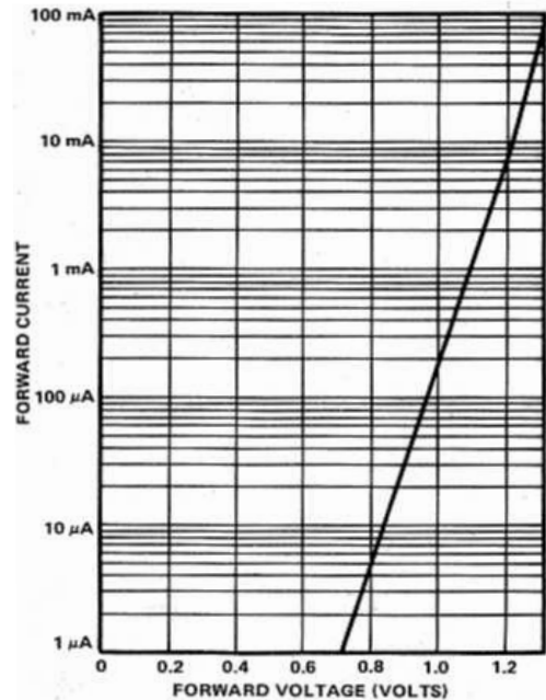
FIGURE 4. Typical Characteristics at 25^{\circ}C Forward Current vs. Forward Voltage (All GaAs PIN Diodes)
