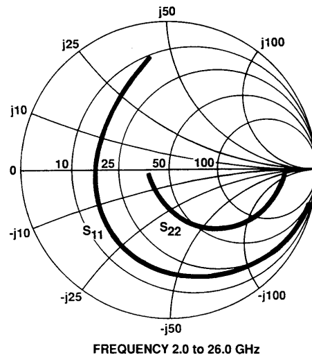
CF004-01 S_{11} AND S_{22} vs FREQUENCY at POWER BIAS V_{DS} = 6\text{ V}, I_{DS} = 25\text{ mA}
