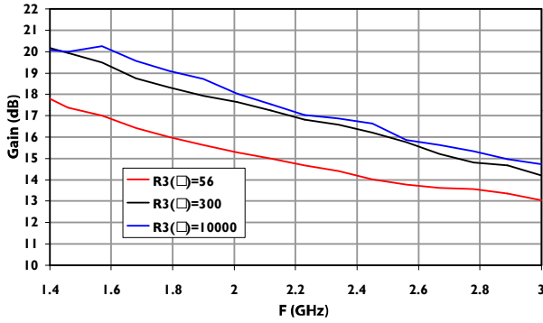
Gain
