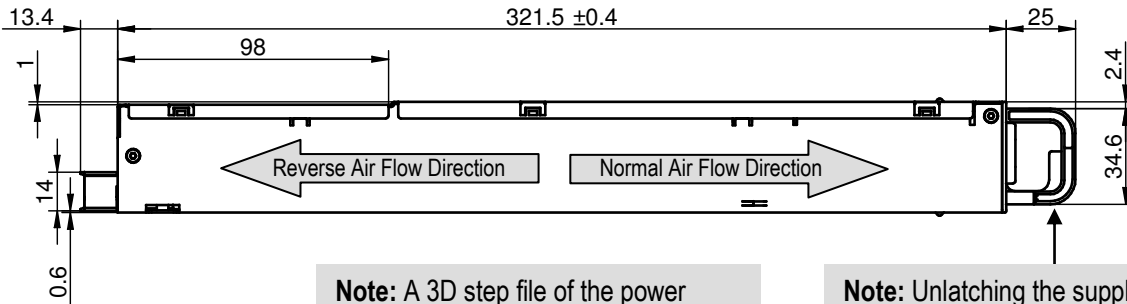
Figure 43: Side view 1
