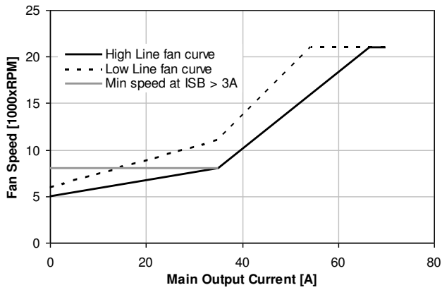
Figure 40: Fan speed vs. main output load for PFE850-12-054RA
