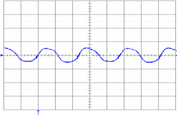
Fig. 22: Output voltage ripple (50 mV/div.) at full rated load current into a resistive load with C_o = 10 \mu\text{F} tantalum + 1\mu\text{F} ceramic and V_{in} = 48 \text{ V} . Time scale: 1 \mu\text{s}/\text{div} .
