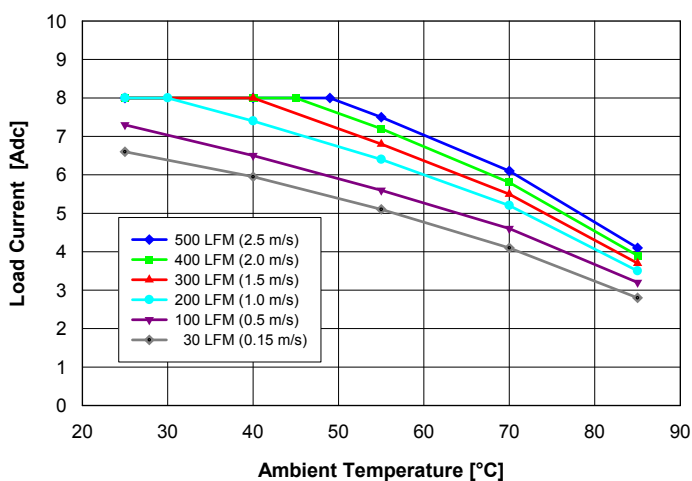
Fig. 13: Available load current vs. ambient temperature and airflow rates for converter mounted horizontally with V_{in} = 54\text{ V} , air flowing from pin 3 to pin 4 and maximum FET temperature \leq 105^{\circ}\text{C} .
