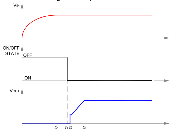
Fig. 8: Start-up scenario #2.
