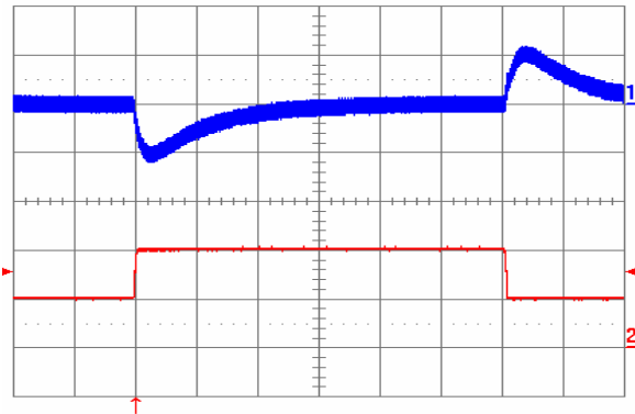
Fig. 20: Output voltage response to load current step-change (2 A – 4 A – 2 A) at V_{in} = 48\text{ V} . Top trace: output voltage (200 mV/div). Bottom trace: load current (2 A/div.). Current slew rate: 0.1 A/ \mu\text{s} . C_o = 1\ \mu\text{F} ceramic. Time scale: 0.5 ms/div.
