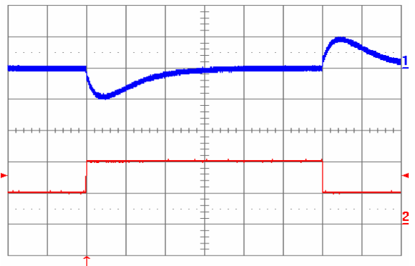
Fig. 21: Output voltage response to load current step-change (2 A – 4 A – 2 A) at V_{in} = 48\text{ V} . Top trace: output voltage (200 mV/div). Bottom trace: load current (2 A/div.). Current slew rate: 5 A/ \mu\text{s} . C_o = 450\ \mu\text{F} tantalum + 1 \mu\text{F} ceramic. Time scale: 0.5 ms/div.
