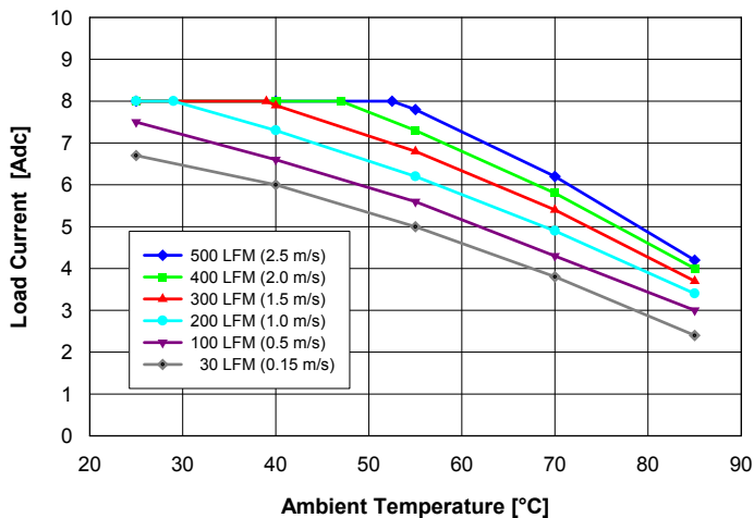
Fig. 11: Available load current vs. ambient air temperature and airflow rates for converter mounted vertically with V_{in} = 54\text{ V} , air flowing from pin 3 to pin 1 and maximum FET temperature \leq 105^{\circ}\text{C} .
