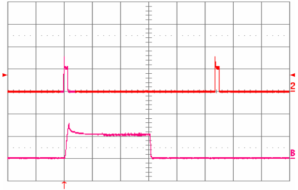
Fig. 27: Load current (top trace, 10 A/div, 20 ms/div) into a 10 m \Omega short circuit during restart, at V_{in} = 48 V. Bottom trace (10 A/div, 1 ms/div) is an expansion of the on-time portion of the top trace.
