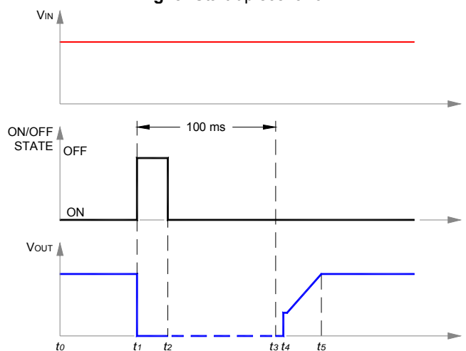
Fig. 9: Start-up scenario #3.
