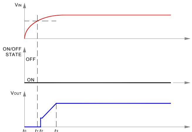
Fig. 7: Start-up scenario #1.
