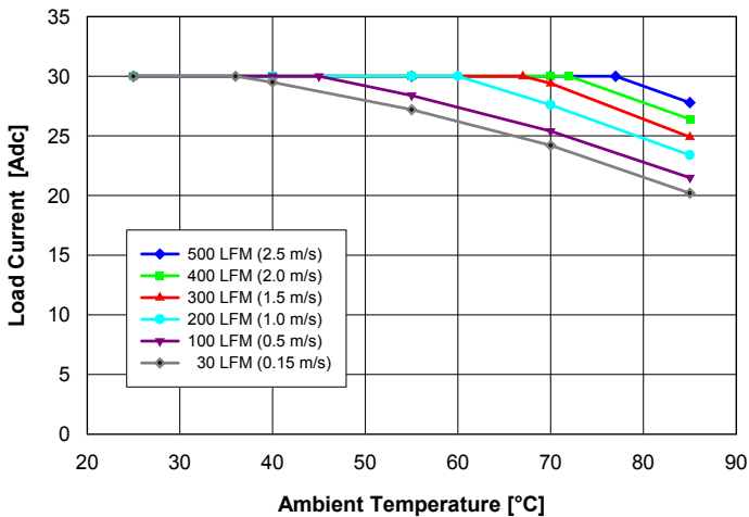
Fig. 1: Available load current vs. ambient air temperature and airflow rates for Q24S30020 converter mounted vertically with air flowing from pin 3 to pin 1, MOSFET temperature \leq 120 °C, V_{in} = 27 V.
