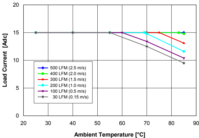
Fig. 1: Available load current vs. ambient air temperature and air-flow rates for Q24T15050 converter mounted vertically with air flowing from pin 3 to pin 1, MOSFET temperature \leq 120^{\circ}\text{C} , V_{in} = 27\text{ V} .
