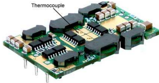
Fig. 28: Location of the thermocouple for thermal testing.
