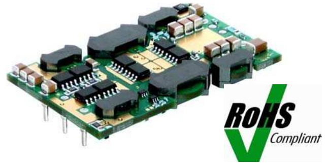
Q24T15050 Converter
