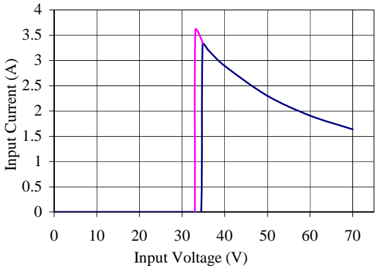
Figure 4. HHS40ZD Input Characteristics
