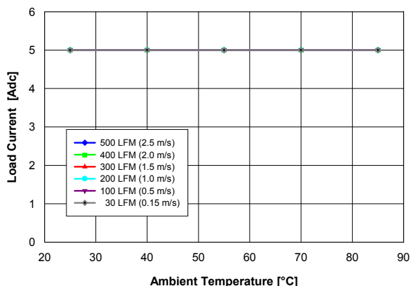
Fig. 2.0V.2: Available load current vs. ambient temperature and airflow rates for V_{out} = 2.0 V converter mounted horizontally with V_{in} = 5 V, air flowing from pin 5 to pin 1 and maximum MOSFET temperature \leq 120 °C.
