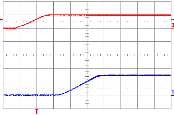
Fig. 1.5V.5: Turn-on transient for V_{out} = 1.5 V with application of V_{in} at full rated load current (resistive) and 47 \mu\text{F} external capacitance at V_{in} = 5 V. Top trace: V_{in} (5 V/div.); Bottom trace: output voltage (1 V/div.); Time scale: 2 ms/div.
