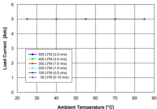
Fig. 2.0V.1: Available load current vs. ambient temperature and airflow rates for V_{out} = 2.0 V converter mounted vertically with V_{in} = 5 V, air flowing from pin 5 to pin 1 and maximum MOSFET temperature \leq 120 °C.
