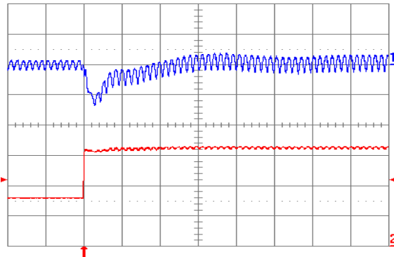
Fig. 3.3V.7: Output voltage response for V_{out} = 3.3\text{ V} to positive load current step change from 2.5\text{ A} to 5\text{ A} with slew rate of 5\text{ A}/\mu\text{s} at V_{in} = 5\text{ V} . Top trace: output voltage ( 100\text{ mV/div.} ); Bottom trace: load current ( 2\text{ A/div.} ). C_o = 47\text{ }\mu\text{F} ceramic + 1\text{ }\mu\text{F} ceramic. Time scale: 20\text{ }\mu\text{s/div.}
