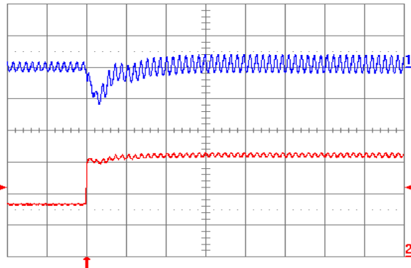
Fig. 1.5V.7: Output voltage response for V_{out} = 1.5 V to positive load current step change from 2.5 A to 5 A with slew rate of 5 \text{ A}/\mu\text{s} at V_{in} = 5 V. Top trace: output voltage (100 mV/div.); Bottom trace: load current (2 A/div.). C_o = 47 \mu\text{F} ceramic + 1 \mu\text{F} ceramic. Time scale: 20 \mu\text{s} /div.
