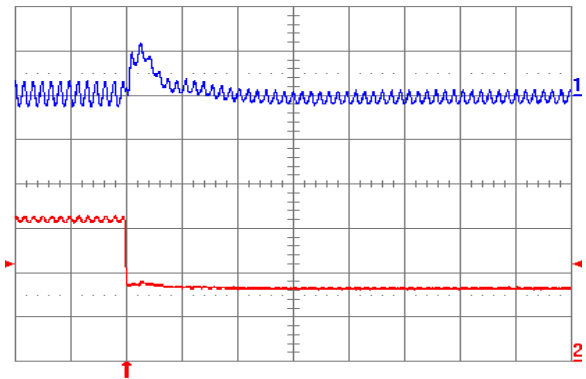
Fig. 1.5V.8: Output voltage response for V_{out} = 1.5 V to negative load current step change from 5 A to 2.5 A with slew rate of -5 \text{ A}/\mu\text{s} at V_{in} = 5 V. Top trace: output voltage (100 mV/div.); Bottom trace: load current (2 A/div.). C_o = 47 \mu\text{F} ceramic + 1 \mu\text{F} ceramic. Time scale: 20 \mu\text{s} /div.
