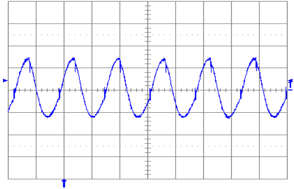
Fig. 1.5V.6: Output voltage ripple (20 mV/div.) at full rated load current into a resistive load with external capacitance 10 \mu\text{F} ceramic + 1 \mu\text{F} ceramic and V_{in} = 5 V for V_{out} = 1.5 V. Time scale: 2 \mu\text{s} /div.
