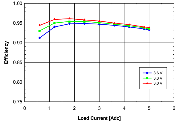
Fig. 2.5V.4: Efficiency vs. load current and input voltage for V_{out} = 2.5 V converter mounted horizontally with air flowing from pin 5 to pin 1 at a rate of 200 LFM (1 m/s) and T_a = 25 °C.
