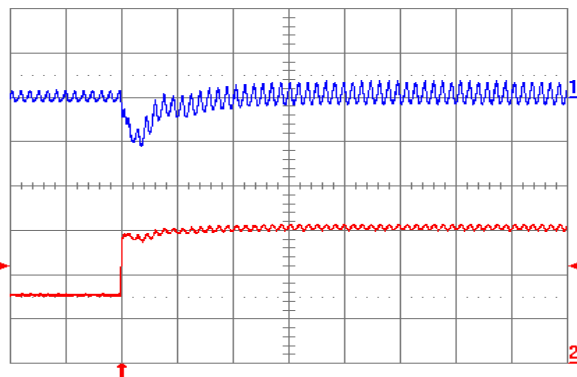
Fig. 1.2V.6: Output voltage response for V_{out} = 1.2\text{ V} to positive load current step change from 2.5\text{ A} to 5\text{ A} with slew rate of 5\text{ A}/\mu\text{s} at V_{in} = 5\text{ V} . Top trace: output voltage ( 100\text{ mV/div.} ); Bottom trace: load current ( 2\text{ A/div.} ). C_o = 47\text{ }\mu\text{F} ceramic + 1\text{ }\mu\text{F} ceramic. Time scale: 20\text{ }\mu\text{s/div.}
