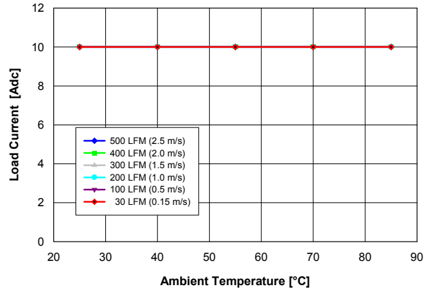
Fig. 2.5V.2: Available load current vs. ambient temperature and airflow rates for Vout = 2.5 V converter mounted horizontally with Vin = 5 V, and maximum MOSFET temperature ≤ 120 °C.
