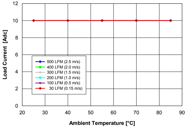
Fig. 1.5V.1: Available load current vs. ambient temperature and airflow rates for Vout = 1.5 V converter mounted vertically with Vin = 5 V, and maximum MOSFET temperature ≤ 120 °C.
