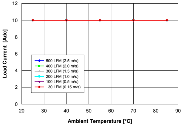
Fig. 2.5V.1: Available load current vs. ambient temperature and airflow rates for Vout = 2.5 V converter mounted vertically with Vin = 5 V, and maximum MOSFET temperature ≤ 120 °C.
