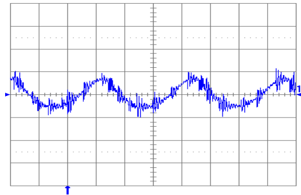
Fig. 3.3V.6: Output voltage ripple (20 mV/div.) at full rated load current into a resistive load with external capacitance 47\ \mu\text{F} ceramic + 1\ \mu\text{F} ceramic, and V_{in} = 5\text{ V} for V_{out} = 3.3\text{ V} . Time scale: 2 \mu\text{s} /div.
