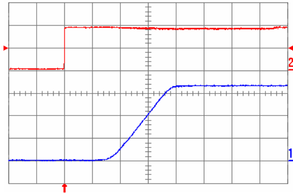
Fig. 3.3V.5: Turn-on transient for V_{out} = 3.3\text{ V} with the application of Enable signal at full rated load current (resistive) and 47\ \mu\text{F} external capacitance at V_{in} = 5\text{ V} . Top trace: Enable signal (2 V/div.); Bottom trace: output voltage (1 V/div.); Time scale: 2 ms/div.
