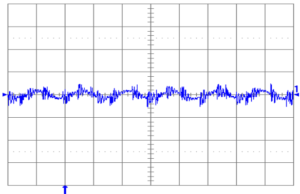
Fig. 2.0V.6: Output voltage ripple (20 mV/div.) at full rated load current into a resistive load with external capacitance 47\ \mu\text{F} ceramic + 1\ \mu\text{F} ceramic, and V_{in} = 5\text{ V} for V_{out} = 2.0\text{ V} . Time scale: 2 \mu\text{s} /div.
