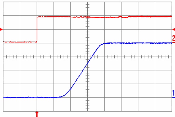
Fig. 2.0V.5: Turn-on transient for V_{out} = 2.0\text{ V} with the application of Enable signal at full rated load current (resistive) and 47\ \mu\text{F} external capacitance at V_{in} = 5\text{ V} . Top trace: Enable signal (2 V/div.); Bottom trace: output voltage (500 mV/div.); Time scale: 2 ms/div.
