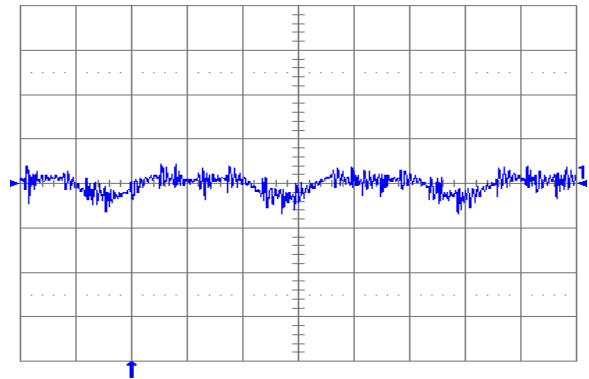
Fig. 1.2V.6: Output voltage ripple (20 mV/div.) at full rated load current into a resistive load with external capacitance 47\text{ }\mu\text{F} ceramic + 1\text{ }\mu\text{F} ceramic, and V_{in} = 5\text{ V} for V_{out} = 1.2\text{ V} . Time scale: 2 \mu\text{s} /div.
