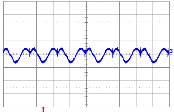
Fig. 1.8V.6: Output voltage ripple ( 20\text{ mV/div.} ) at full rated load current into a resistive load with external capacitance 100\text{ }\mu\text{F} ceramic + 1\text{ }\mu\text{F} ceramic, and V_{in} = 12\text{ V} for V_{out} = 1.8\text{ V} . Time scale: 2\text{ }\mu\text{s/div.}
