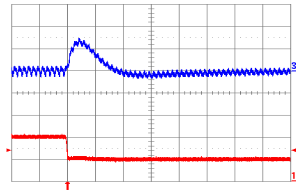
Fig. 3.3V.8: Output voltage response for V_{out} = 3.3 V to negative load current step change from 10 A to 5 A with slew rate of -5 \text{ A}/\mu\text{s} at V_{in} = 12 V. Top trace: output voltage (100 mV/div.); Bottom trace: load current (2 A/div.). C_o = 100 \mu\text{F} ceramic. Time scale: 20 \mu\text{s}/\text{div} .
