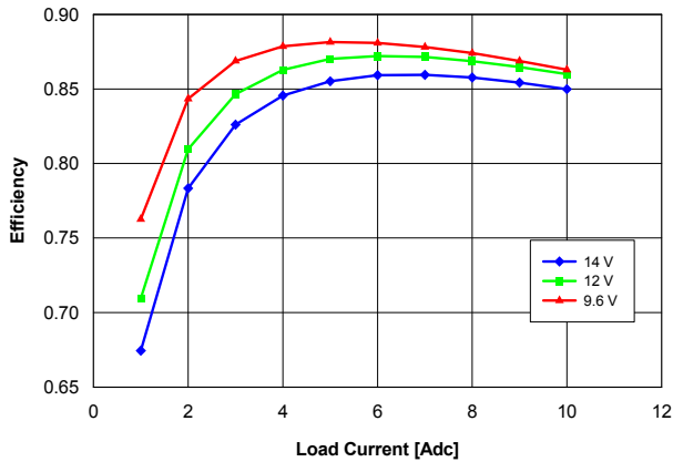
Fig. 1.0V.3: Efficiency vs. load current and input voltage for V_{out} = 1.0 V converter mounted vertically with air flowing at a rate of 200 LFM (1 m/s) and T_a = 25 °C.
