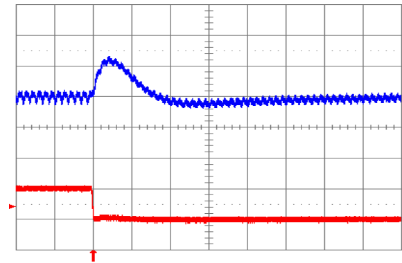
Fig. 2.5V.8: Output voltage response for V_{out} = 2.5\text{ V} to negative load current step change from 10 A to 5 A with slew rate of -5\text{ A}/\mu\text{s} at V_{in} = 12\text{ V} . Top trace: output voltage (100 mV/div.); Bottom trace: load current (5 A/div.). C_o = 100\text{ }\mu\text{F} ceramic. Time scale: 20 \mu\text{s} /div.
