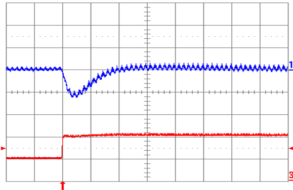
Fig. 2.0V.7: Output voltage response for V_{out} = 2.0 V to positive load current step change from 5 A to 10 A with slew rate of 5 \text{ A}/\mu\text{s} at V_{in} = 12 V. Top trace: output voltage (100 mV/div.); Bottom trace: load current (5 A/div.); C_o = 100 \mu\text{F} ceramic. Time scale: 20 \mu\text{s}/\text{div} .
