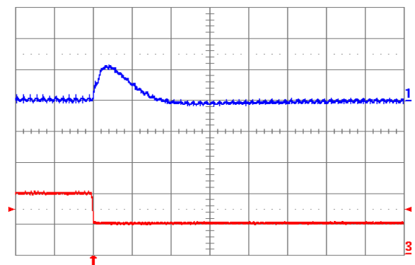
Fig. 0.7525V.8: Output voltage response for V_{out} = 0.7525 V to negative load current step change from 10 A to 5 A with slew rate of -5 A/ \mu\text{s} at V_{in} = 12 V. Top trace: output voltage (100 mV/div.); Bottom trace: load current (5 A/div.). C_o = 100 \mu\text{F} ceramic. Time scale: 20 \mu\text{s} /div.
