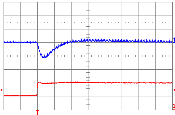
Fig. 0.7525V.7: Output voltage response for V_{out} = 0.7525 V to positive load current step change from 5 A to 10 A with slew rate of 5 A/ \mu\text{s} at V_{in} = 12 V. Top trace: output voltage (100 mV/div.); Bottom trace: load current (5 A/div.). C_o = 100 \mu\text{F} ceramic. Time scale: 20 \mu\text{s} /div.
