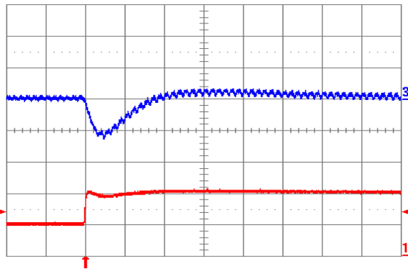
Fig. 1.2V.7: Output voltage response for V_{out} = 1.2 V to positive load current step change from 5 A to 10 A with slew rate of 5 \text{ A}/\mu\text{s} at V_{in} = 12 V. Top trace: output voltage (100 mV/div.); Bottom trace: load current (5 A/div.). C_o = 100 \mu\text{F} ceramic. Time scale: 20 \mu\text{s} /div.
