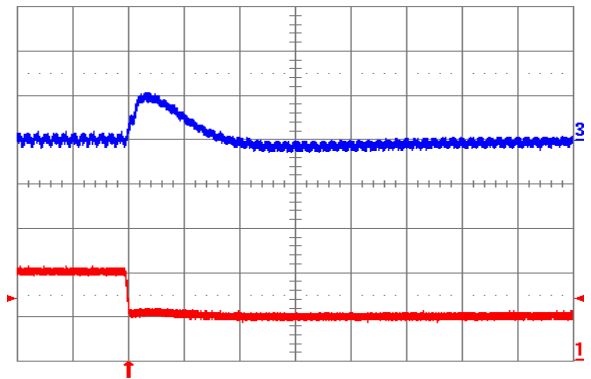
Fig. 1.2V.8: Output voltage response for V_{out} = 1.2 V to negative load current step change from 10 A to 5 A with slew rate of -5 \text{ A}/\mu\text{s} at V_{in} = 12 V. Top trace: output voltage (100 mV/div.); Bottom trace: load current (5 A/div.). C_o = 100 \mu\text{F} ceramic. Time scale: 20 \mu\text{s} /div.
