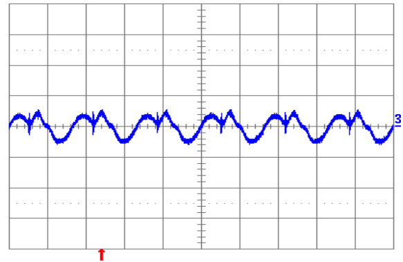
Fig. 1.5V.6: Output voltage ripple (20 mV/div.) at full rated load current into a resistive load with external capacitance 100 \mu\text{F} ceramic + 1 \mu\text{F} ceramic, and V_{in} = 12 V for V_{out} = 1.5 V. Time scale: 2 \mu\text{s} /div.
