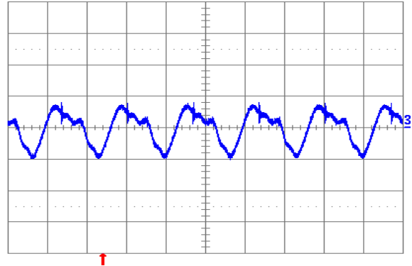
Fig. 3.3V.6: Output voltage ripple (20 mV/div.) at full rated load current into a resistive load with external capacitance 100 \mu\text{F} ceramic + 1 \mu\text{F} ceramic, and V_{in} = 12 V for V_{out} = 3.3 V. Time scale: 2 \mu\text{s}/\text{div} .
