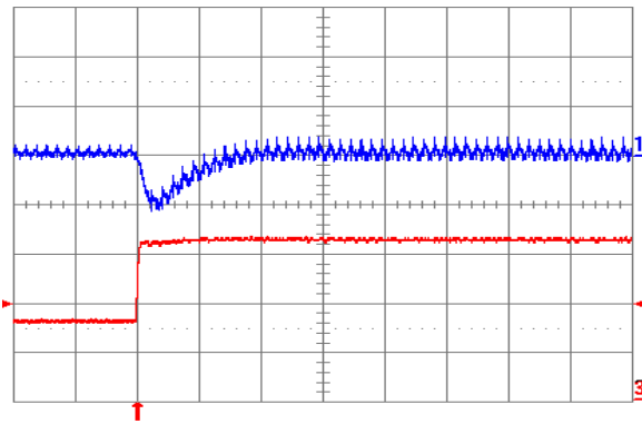
Fig. 5.0V.6: Output voltage response for V_{out} = 5.0\text{ V} to positive load current step change from 8 A to 16 A with slew rate of 5\text{ A}/\mu\text{s} at V_{in} = 12\text{ V} . Top trace: output voltage (200 mV/div.); Bottom trace: load current (5A/div.). C_o = 100\ \mu\text{F} ceramic. Time scale: 20 \mu\text{s} /div.
