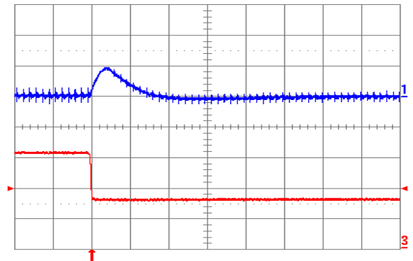
Fig. 0.7525V.7: Output voltage response for V_{out} = 0.7525\ \text{V} to negative load current step change from 16 A to 8 A with slew rate of -5\ \text{A}/\mu\text{s} at V_{in} = 12\ \text{V} . Top trace: output voltage (200 mV/div.); Bottom trace: load current (5 A/div.). C_o = 100\ \mu\text{F} ceramic. Time scale: 20 \mu\text{s} /div.
