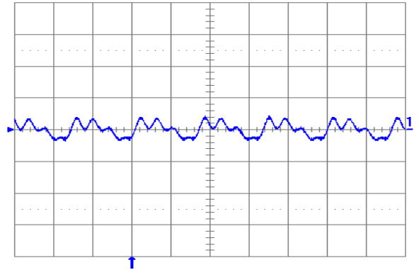
Fig. 2.0V.5: Output voltage ripple (20 mV/div.) at full rated load current into a resistive load with external capacitance 100\ \mu\text{F} ceramic + 1\ \mu\text{F} ceramic and V_{in} = 12\text{ V} for V_{out} = 2.0\text{ V} . Time scale: 2 \mu\text{s} /div.
