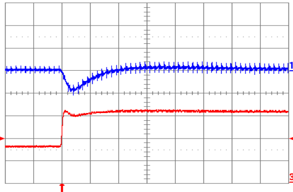
Fig. 0.7525V.6: Output voltage response for V_{out} = 0.7525\ \text{V} to positive load current step change from 8 A to 16 A with slew rate of 5\ \text{A}/\mu\text{s} at V_{in} = 12\ \text{V} . Top trace: output voltage (200 mV/div.); Bottom trace: load current (5 A/div.). C_o = 100\ \mu\text{F} ceramic. Time scale: 20 \mu\text{s} /div.
