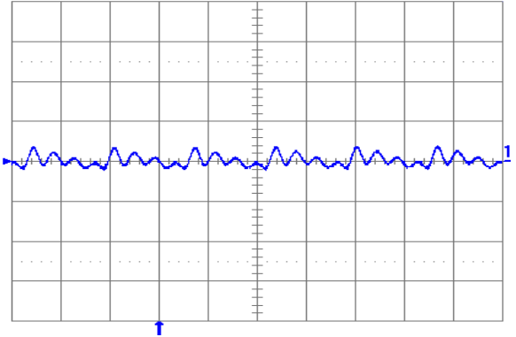
Fig. 0.7525V.5: Output voltage ripple (20 mV/div.) at full rated load current into a resistive load with external capacitance 100\ \mu\text{F} ceramic + 1\ \mu\text{F} ceramic and V_{in} = 12\ \text{V} for V_{out} = 0.7525\ \text{V} . Time scale: 2 \mu\text{s} /div.
