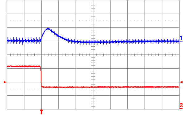
Fig. 1.0V.7: Output voltage response for V_{out} = 1.0 V to negative load current step change from 16 A to 8 A with slew rate of -5 \text{ A}/\mu\text{s} at V_{in} = 12 V. Top trace: output voltage (200 mV/div.); Bottom trace: load current (5 A/div.). C_o = 100 \mu\text{F} ceramic. Time scale: 20 \mu\text{s} /div.
