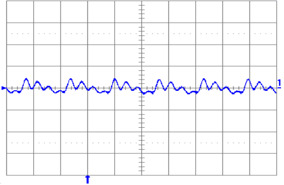
Fig. 1.5V.5: Output voltage ripple (20 mV/div.) at full rated load current into a resistive load with external capacitance 100\ \mu\text{F} ceramic + 1\ \mu\text{F} ceramic and V_{in} = 12\text{ V} for V_{out} = 1.5\text{ V} . Time scale: 2 \mu\text{s} /div.
