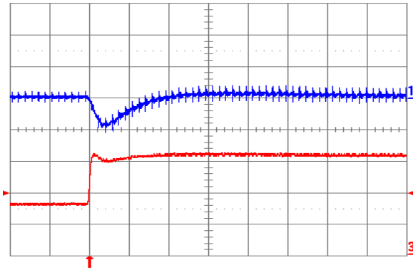
Fig. 1.0V.6: Output voltage response for V_{out} = 1.0 V to positive load current step change from 8 A to 16 A with slew rate of 5 \text{ A}/\mu\text{s} at V_{in} = 12 V. Top trace: output voltage (200 mV/div.); Bottom trace: load current (5 A/div.). C_o = 100 \mu\text{F} ceramic. Time scale: 20 \mu\text{s} /div.
