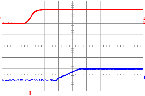
Fig. 0.7525V.4: Turn-on transient for V_{out} = 0.7525\text{V} with application of V_{in} at full rated load current (resistive) and 100\ \mu\text{F} external capacitance at V_{in} = 12\ \text{V} . Top trace: V_{in} (10 V/div.); Bottom trace: output voltage (1 V/div.); Time scale: 2 ms/div.
