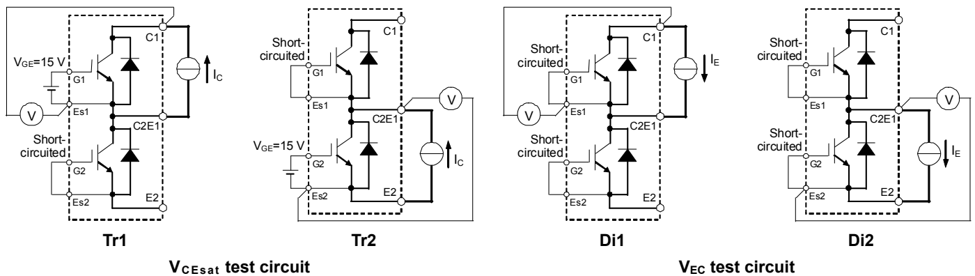
Tr1/Tr2: IGBT, Di1/Di2: FWDi
